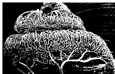
Digestiver Tinnitus
